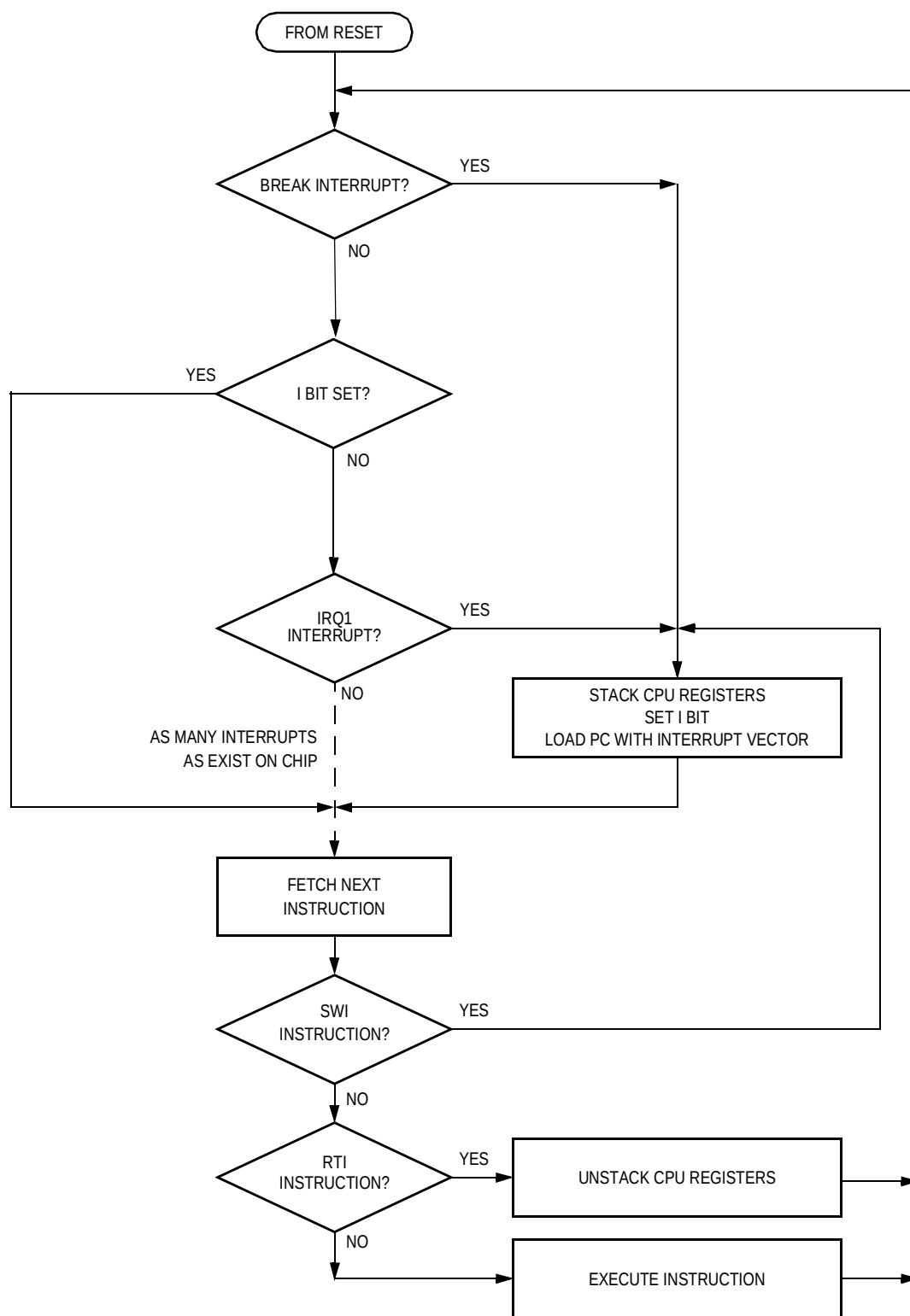
Figure 9-10. Interrupt Processing
