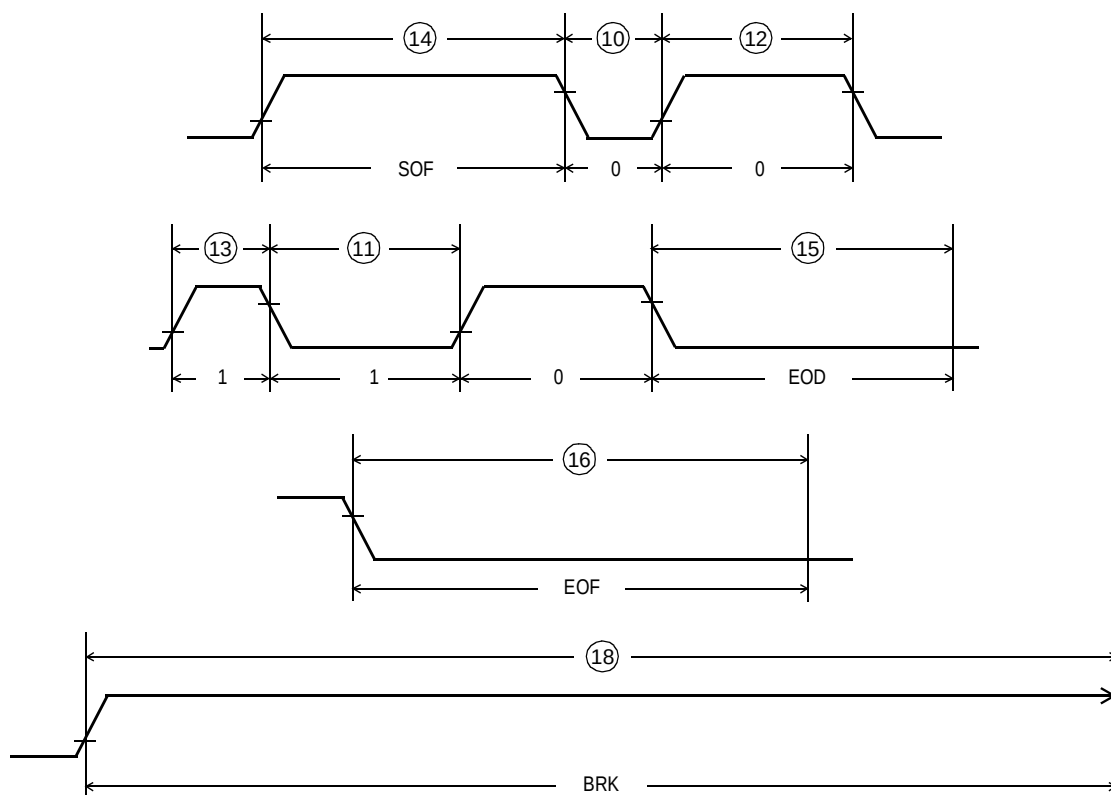
Figure 24-3. BDL Variable Pulse-Width Modulation (VPW) Symbol Timing
