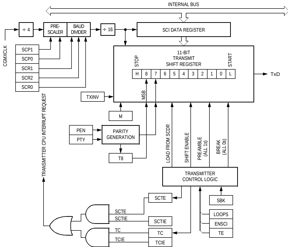
Figure 17-4. SCI Transmitter
