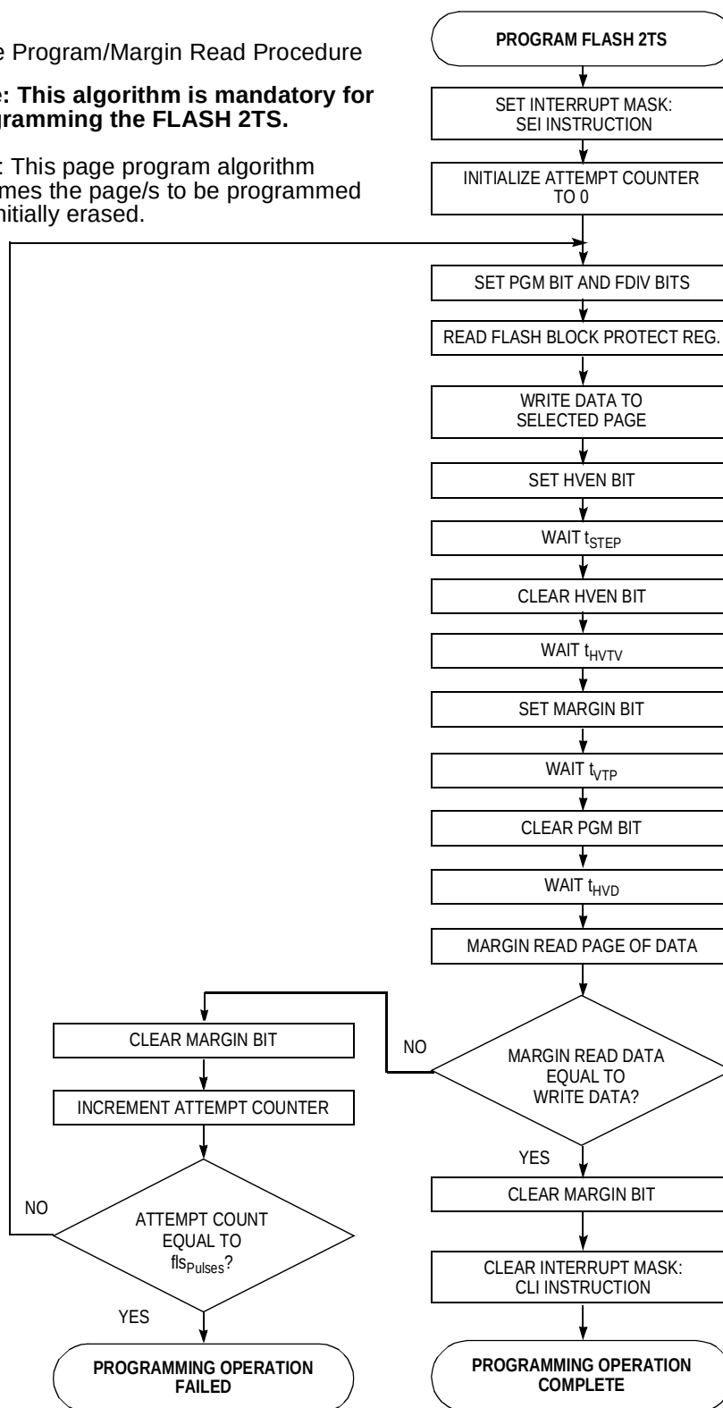
Figure 5-2. Smart Programming Algorithm
