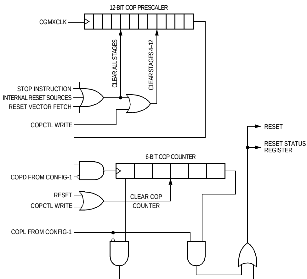
Figure 14-1. COP Block Diagram
