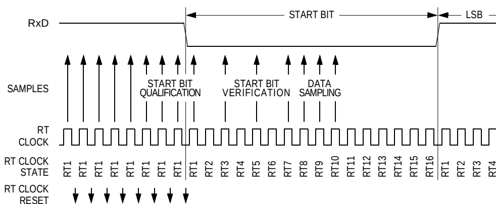
Figure 17-6. Receiver Data Sampling
