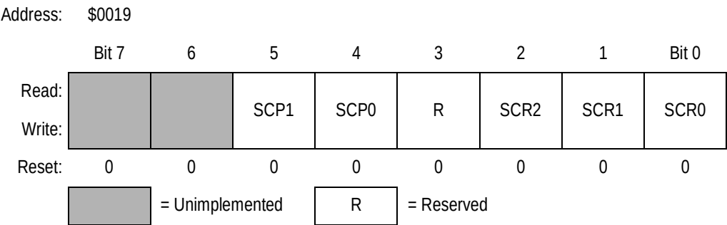
Figure 17-16. SCI Baud Rate Register (SCBR)
