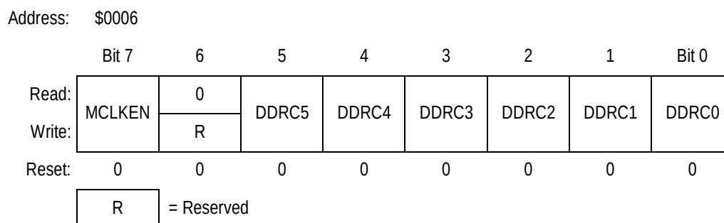
Figure 20-9. Data Direction Register C (DDRC)
