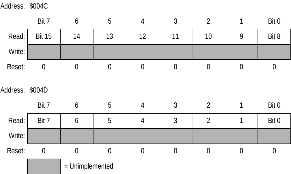
Figure 19-4. TIM Counter Registers (TCNTH–TCNTL)
