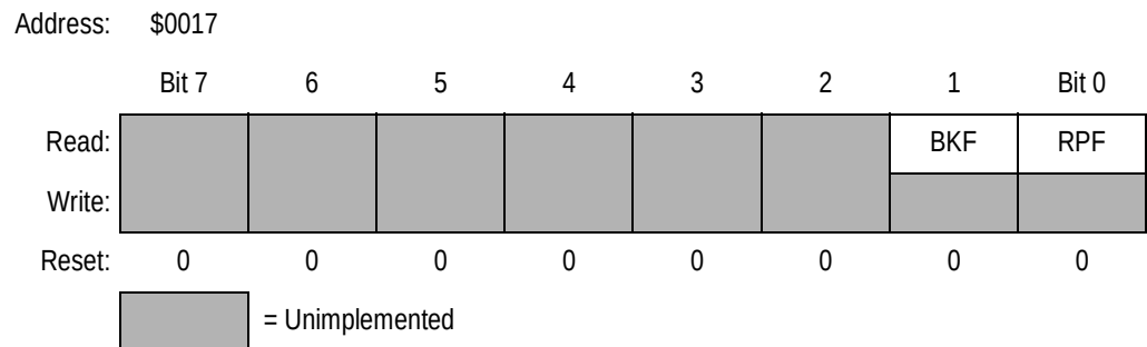
Figure 17-14. SCI Status Register 2 (SCS2)
