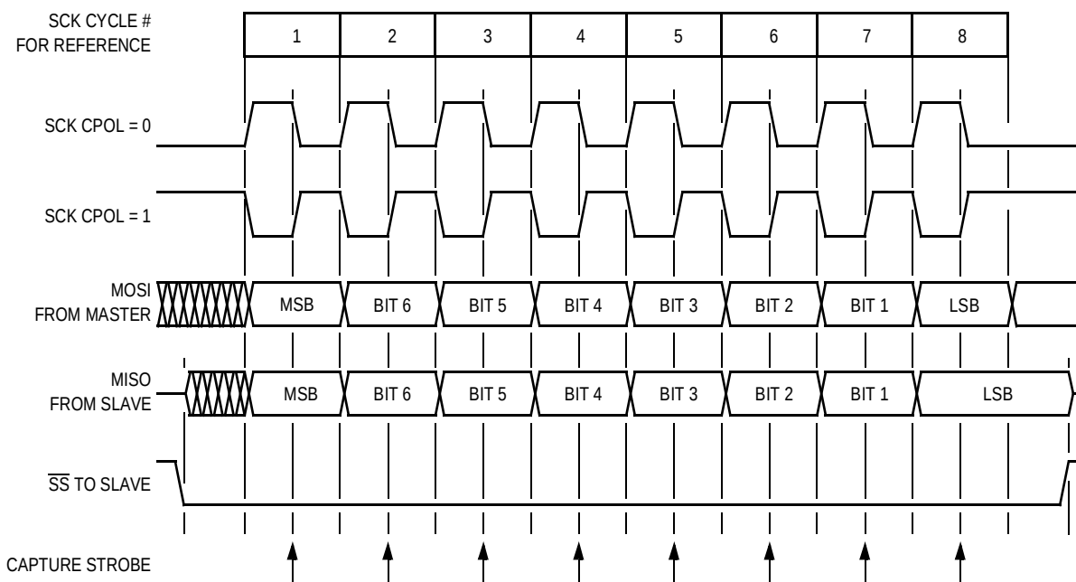
Figure 18-5. Transmission Format (CPHA = 1)
