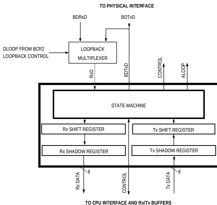
Figure 21-14. BDLC Protocol Handler Outline
