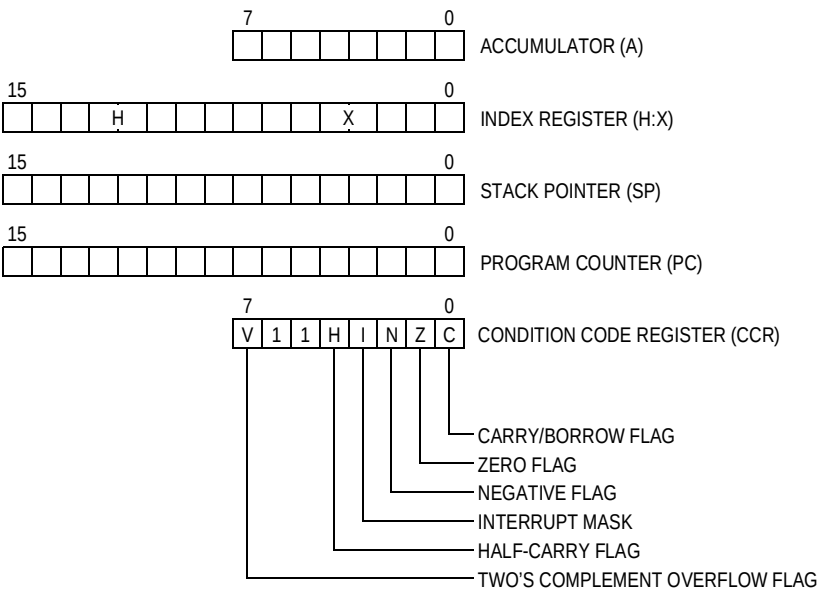
Figure 8-1. CPU Registers
