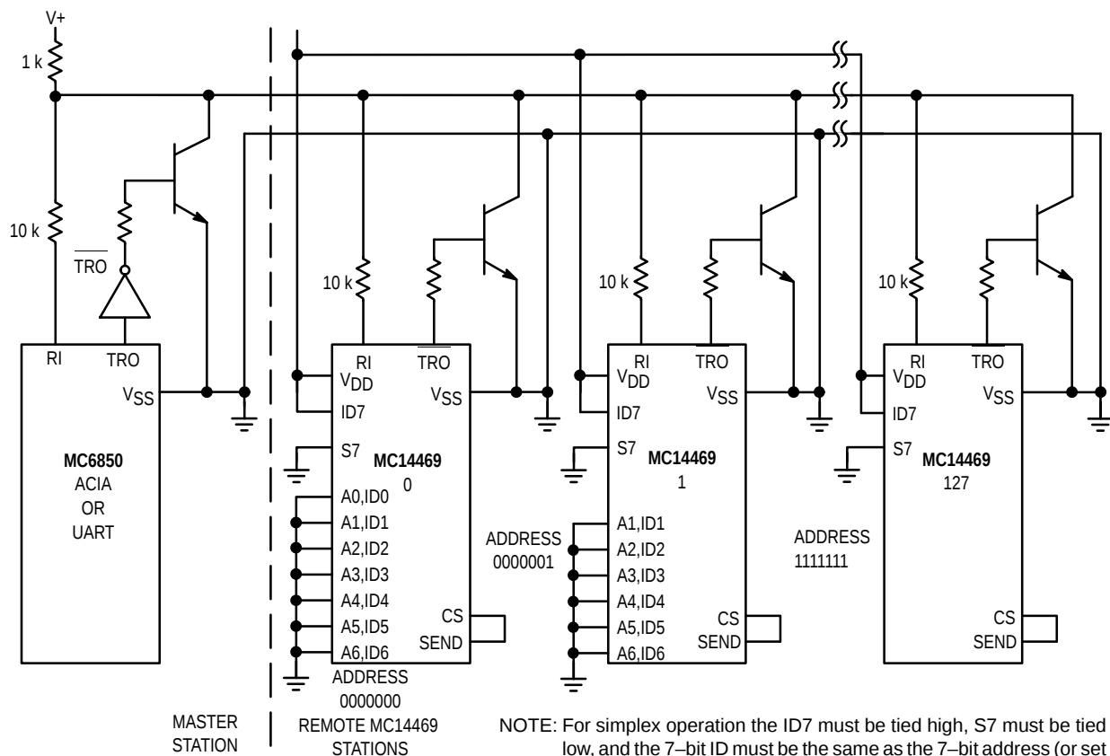
Figure 6. Single Line, Simplex Data Transmission
