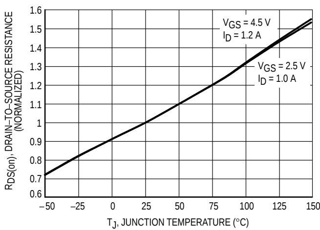
Figure 5. On-Resistance Variation Over Temperature
