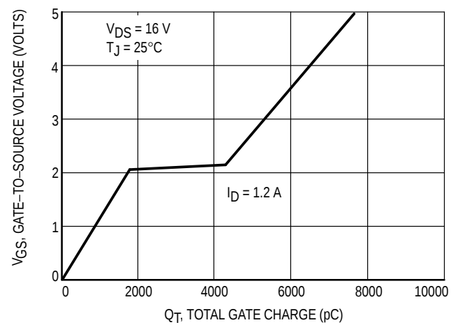
Figure 6. Gate Charge
