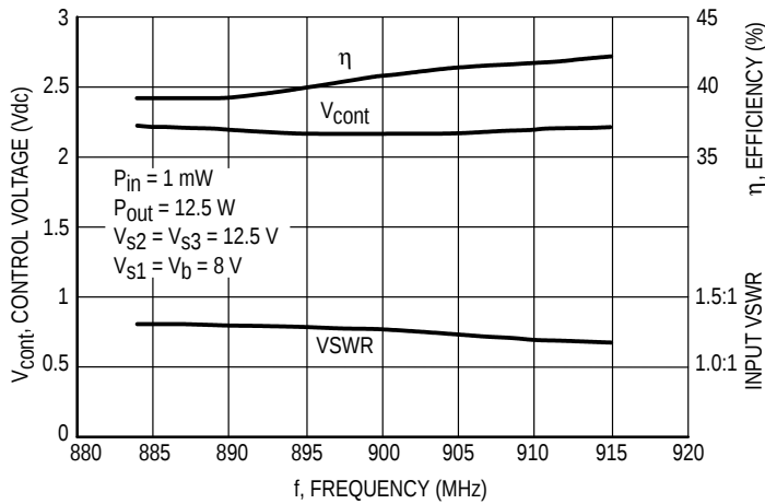
Figure 2. Control Voltage, Efficiency and Input VSWR versus Frequency
