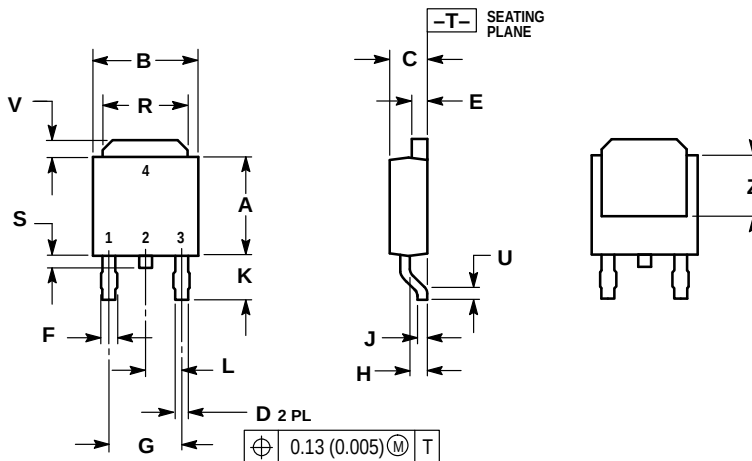
CASE 369A-13 ISSUE W
