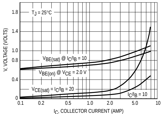
Figure 9. "On" Voltage
