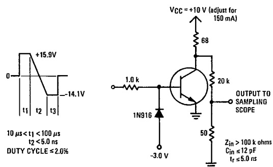
FIGURE 2 — TURN-OFF TIME TEST CIRCUIT
