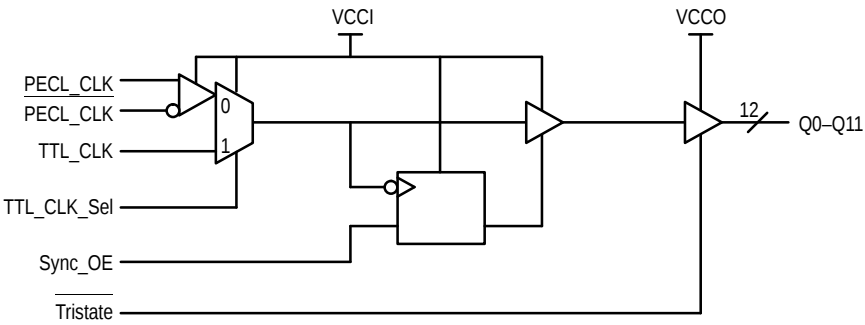
Figure 1. Logic Diagram
