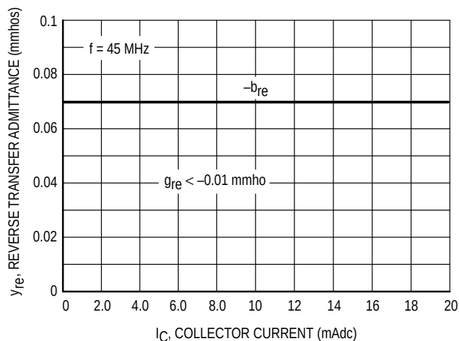
Figure 4. Reverse Transfer Admittance
