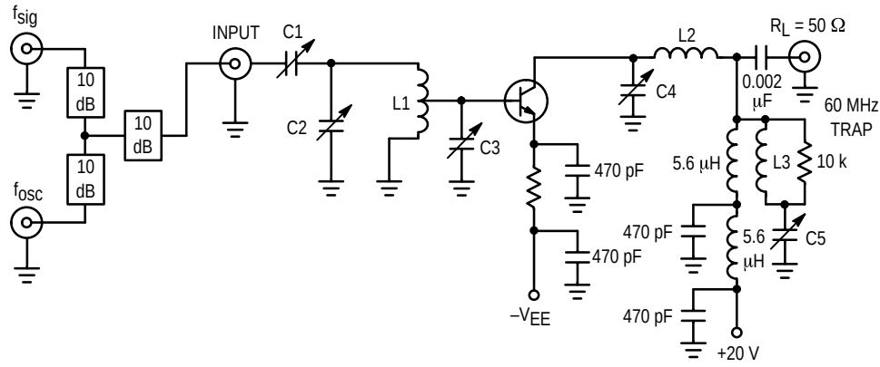
Figure 7. VHF Mixer Test Circuit ( f_{if} = 44 \text{ MHz} , B.W. = 6.0 MHz)
