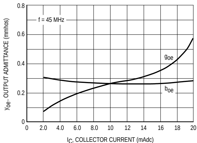
Figure 6. Output Admittance
