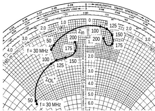
Figure 10. Series Equivalent Input-Output Impedance
