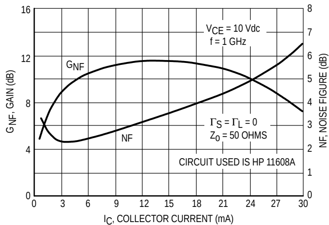
Figure 2. Gain and Noise Figure versus Collector Current
