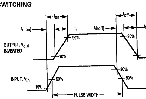
Figure 14. Switching Waveforms
