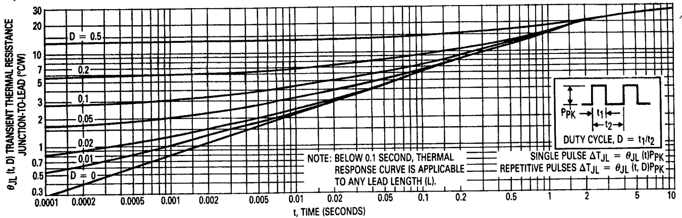
Figure 2. Typical Thermal Response L, Lead Length = 3/8 Inch
