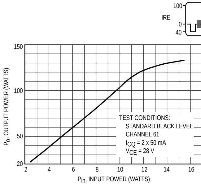
Figure 5. Peak Output Power versus Peak Input Power
