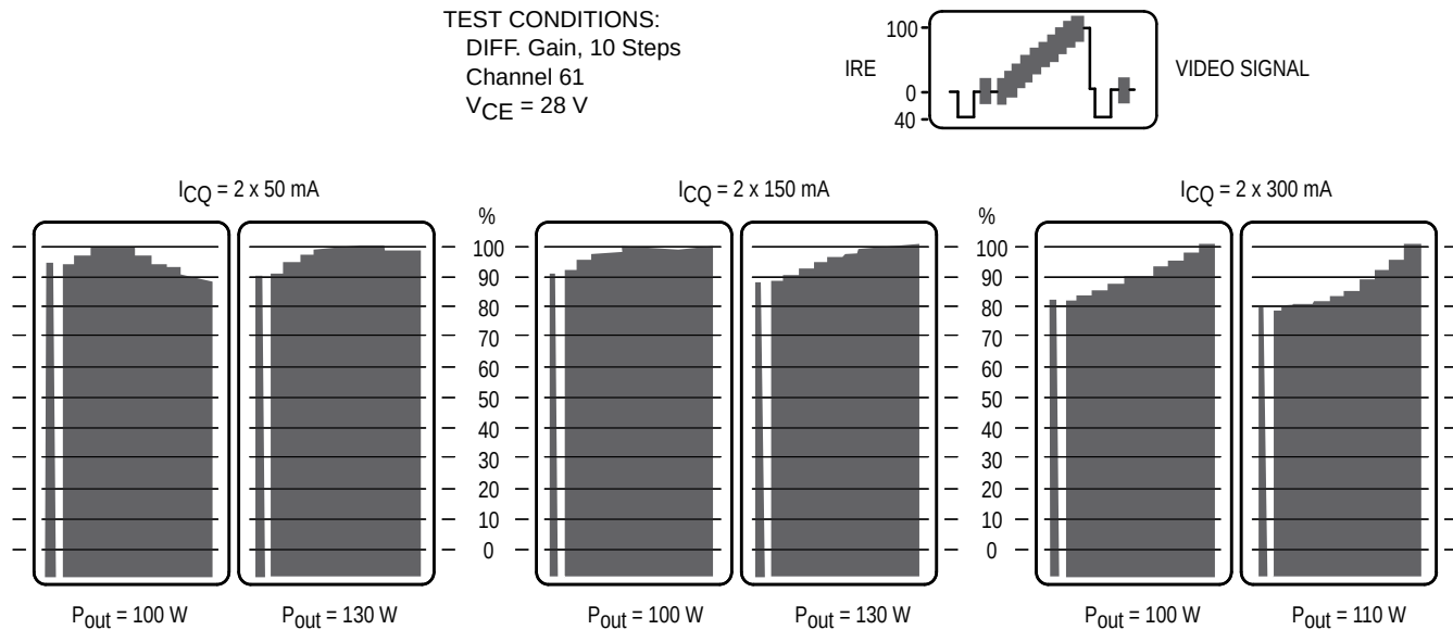
Figure 7. Gain versus Output Power
