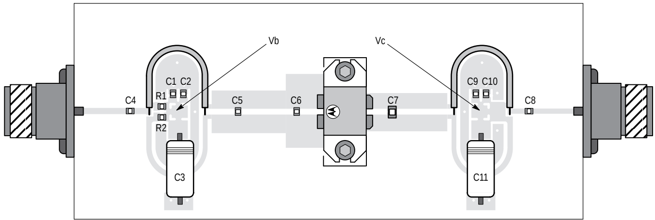
Figure 10. Components View
