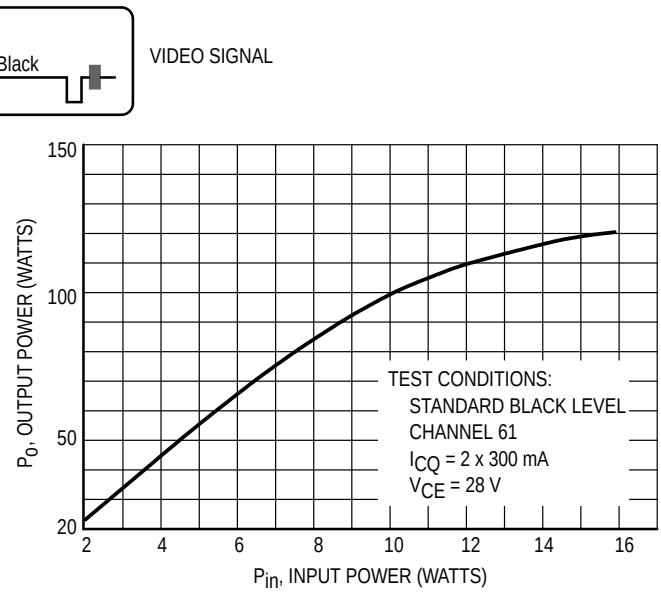
Figure 6. Peak Output Power versus Peak Input Power
