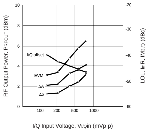
RF OUTPUT POWER vs. I/Q INPUT VOLTAGE
