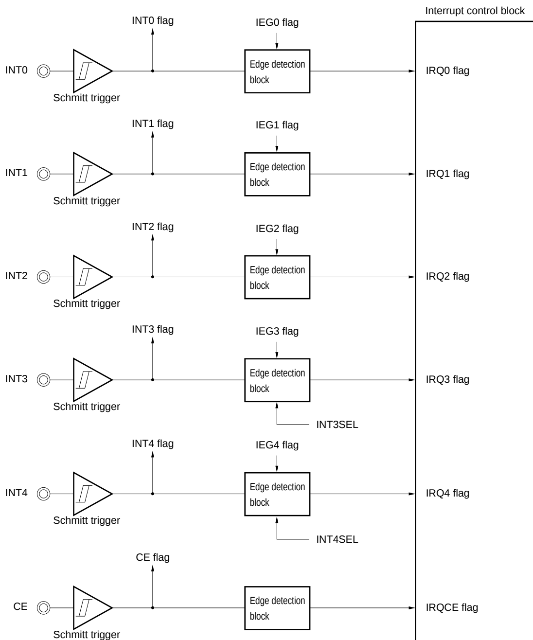
Figure 12-20. Outline of External Interrupts
