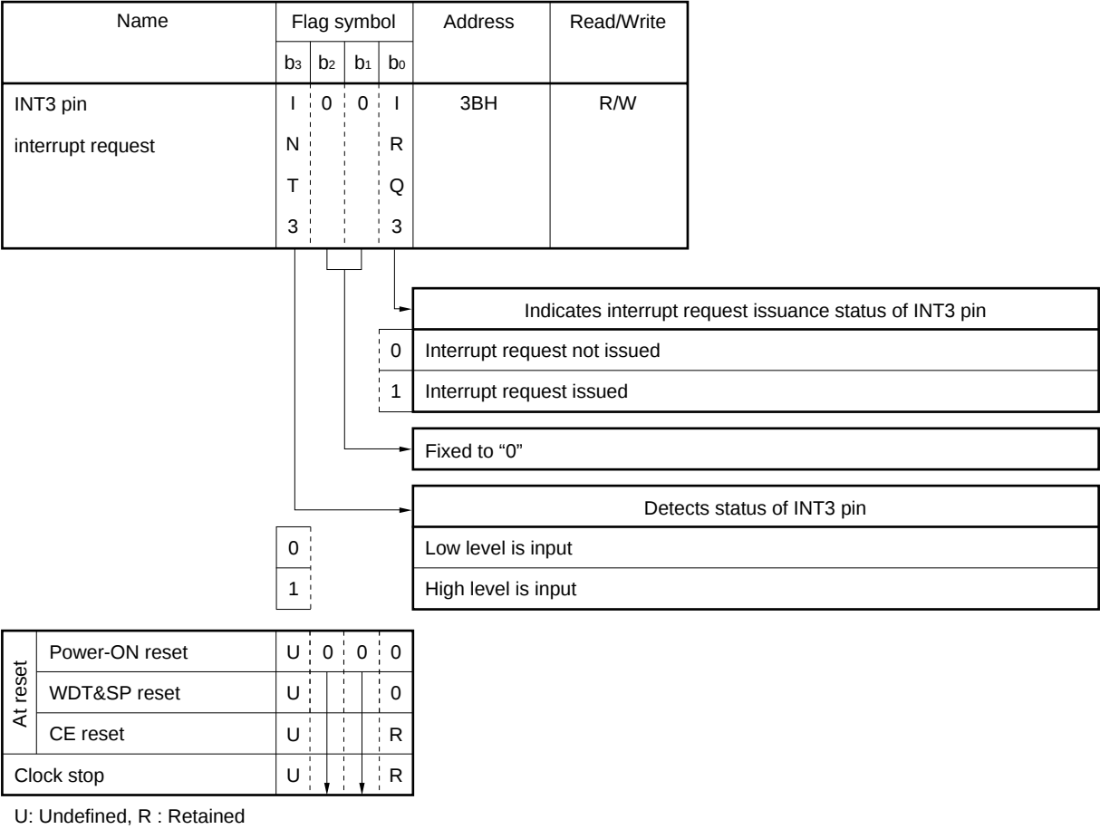
Figure 12-9. Configuration of INT3 Pin Interrupt Request Register
