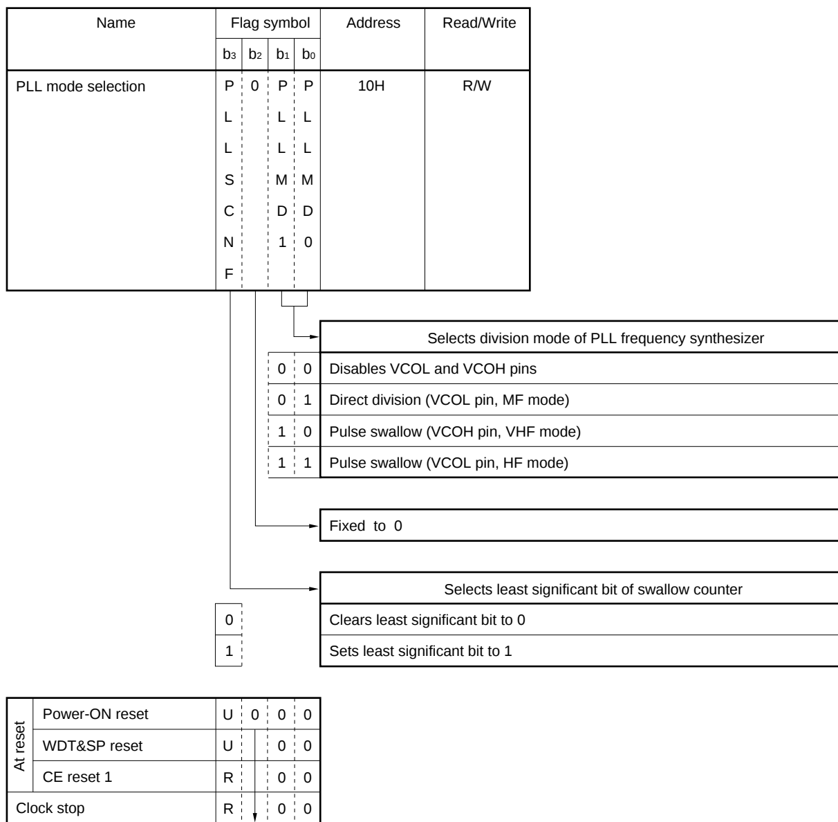
Figure 17-3. Configuration of PLL Mode Selection Register
