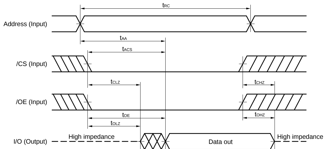
Read Cycle Timing Chart 2 (/CS Access)
