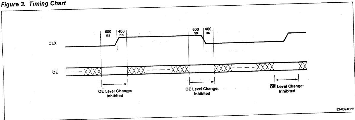
Figure 3. Timing Chart
