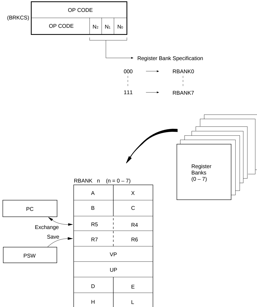
Figure 4-4. Context Switching by Execution of BRKCS Instruction
