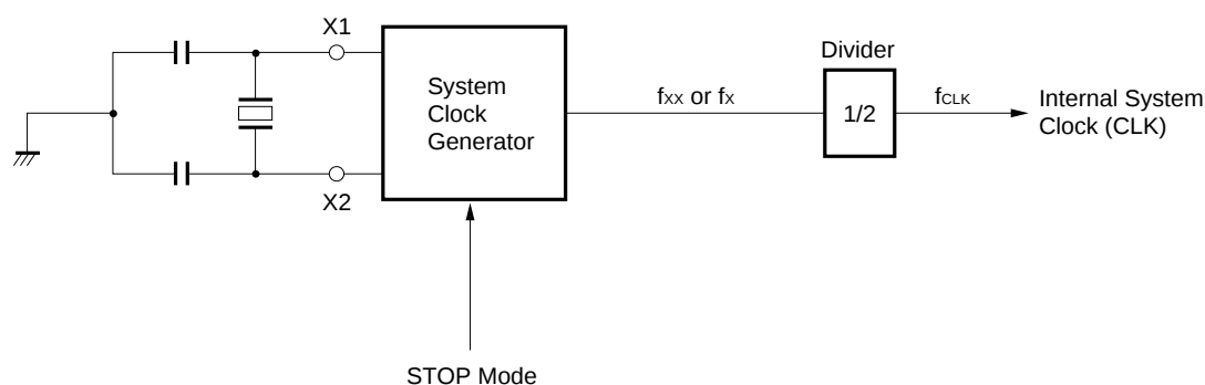
Figure 3-1. Clock Generator Block Diagram
