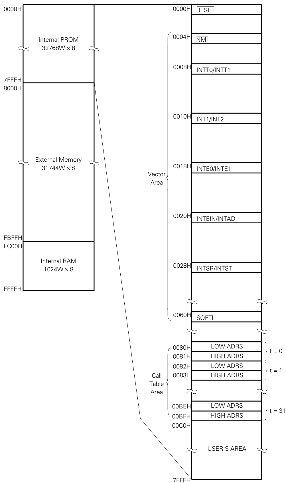
Figure 2-4. Memory Map ( \mu PD78C18 Mode)
