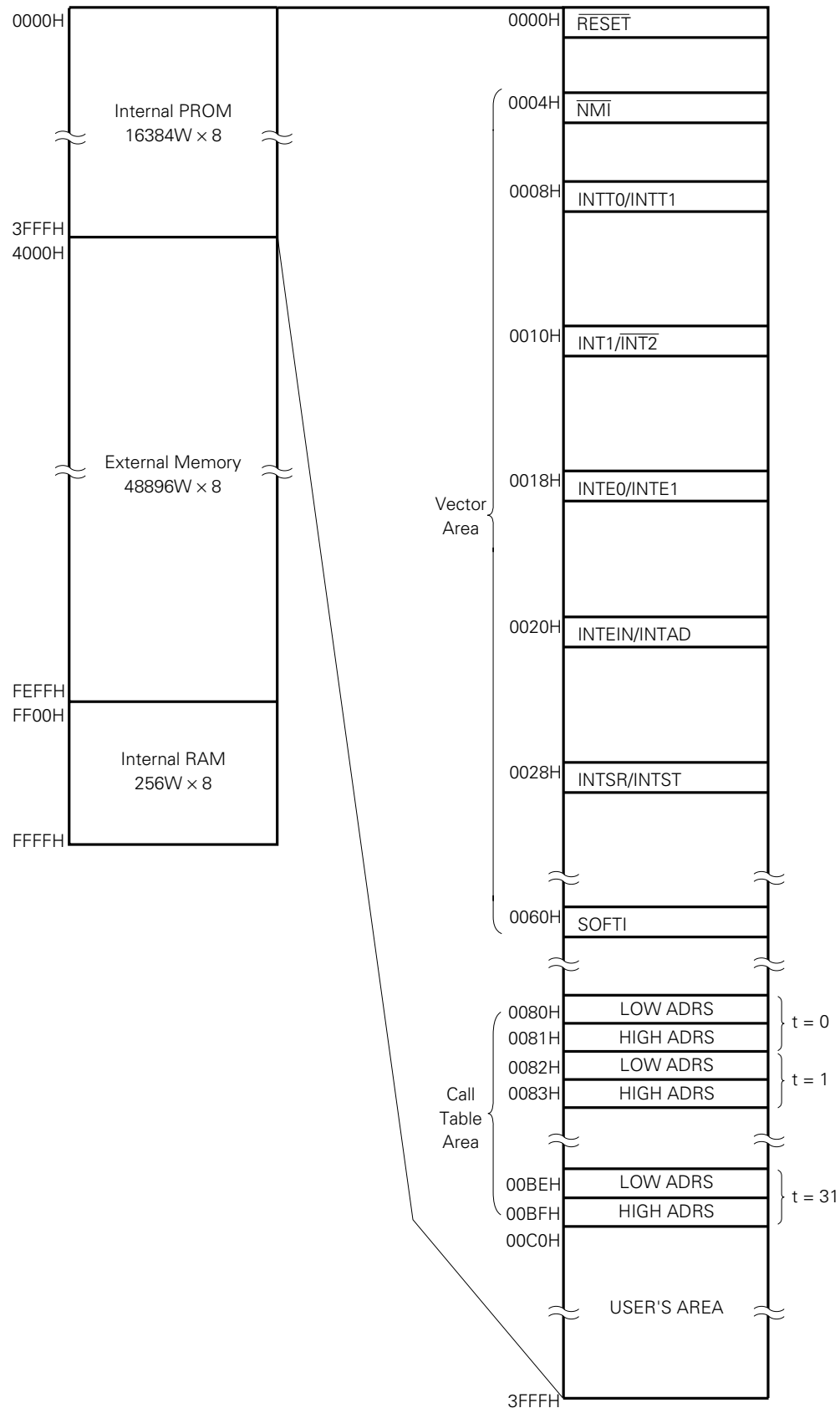
Figure 2-3. Memory Map ( \mu PD78C14 Mode)
