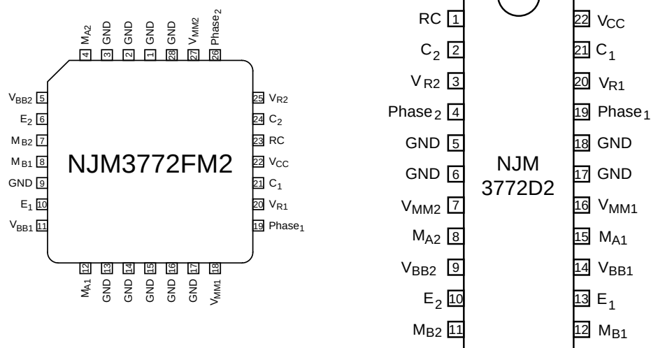
Figure 2. Pin configurations
