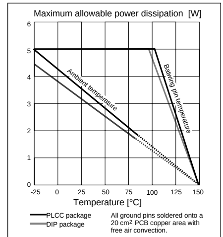
Figure 11. Maximum allowable power dissipation vs. temperature
