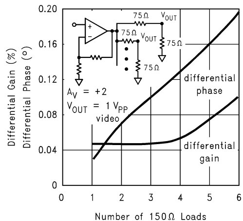
Differential Gain and Phase vs. Load
