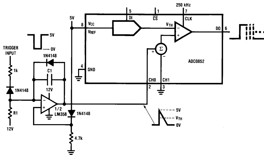
FIGURE 17. Pulse-Width Modulator
