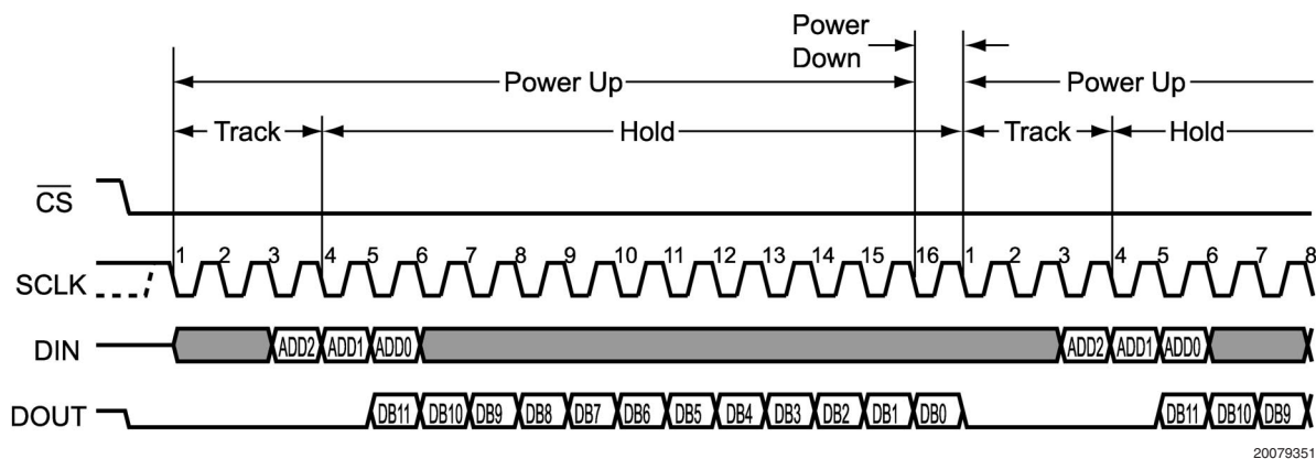
FIGURE 1. ADC78H90 Operational Timing Diagram
