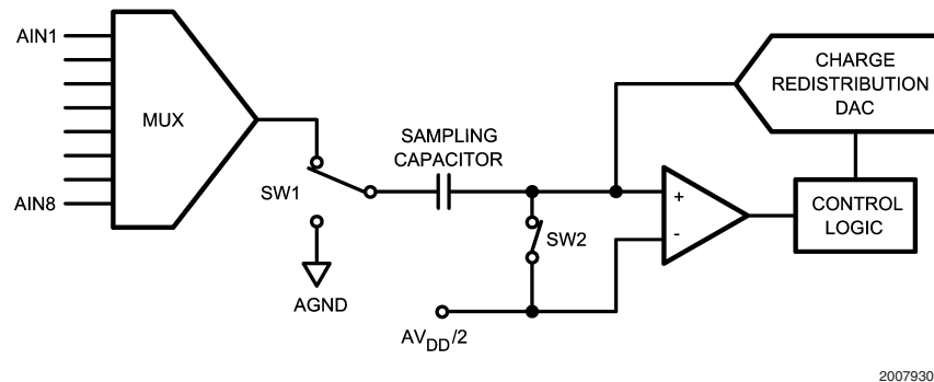
FIGURE 2. ADC78H90 in Track Mode
