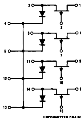
AH5011C and AH5012C SPST Switches (Quad Version Shown) Order Number AH5011CM, AH5011CN, AH5012CM or AH5012CN See NS Package Number M16A or N16A
