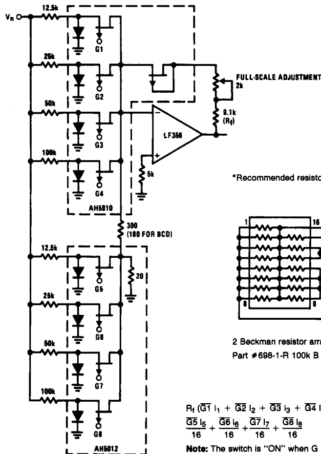
8-Bit Binary (BCD) Multiplying D/A Converter*
