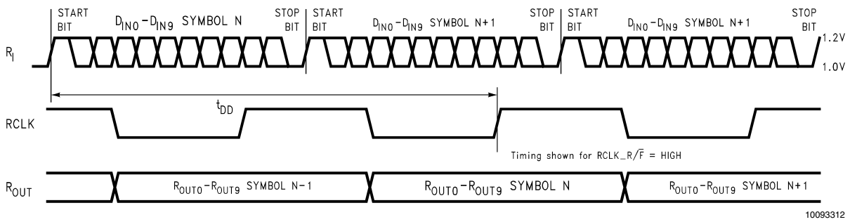
FIGURE 12. Deserializer Delay
