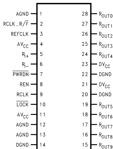
DS92LV1224TMSA - Deserializer
