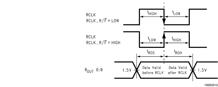
FIGURE 13. Deserializer Data Valid Out Times
