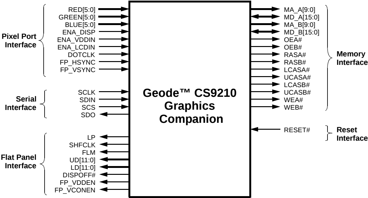
Figure 2-1. CS9210 Signal Groups
