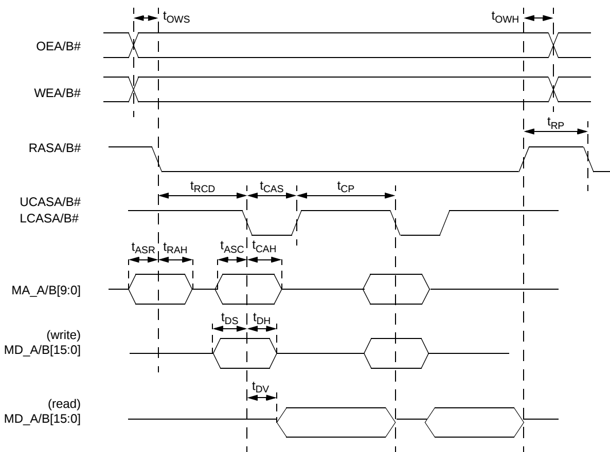
Figure 5-5. Memory Interface Signals
