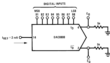
FIGURE 5. Basic Negative Reference Operation (Note 5)
