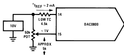
FIGURE 4. Recommended Full Scale Adjustment Circuit (Note 5)
