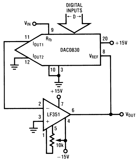
DAC Controlled Amplifier (Volume Control)
