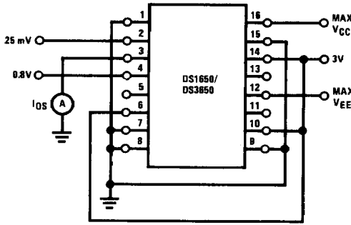
FIGURE 4. I_{OS}
