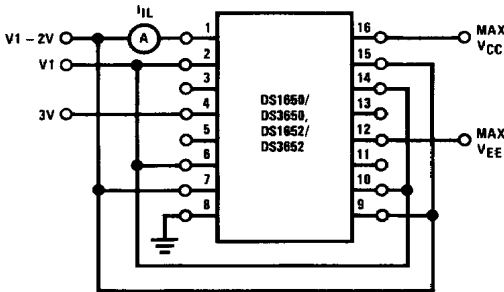
FIGURE 6. I_{IL}
