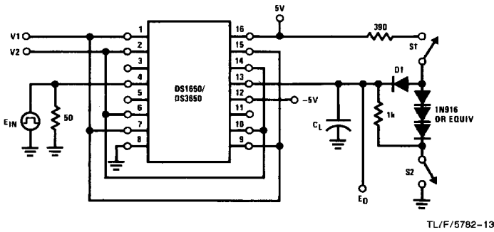
FIGURE 8. Receiver Propagation Delay t_{PLH(D)} and t_{PHL(D)}
