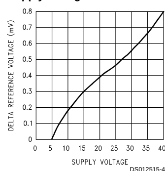
\Delta Reference Voltage vs Supply Voltage
