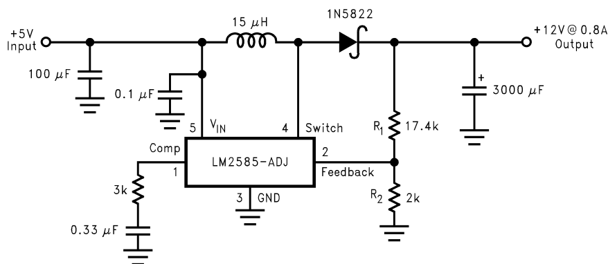
FIGURE 38. Boost Regulator
