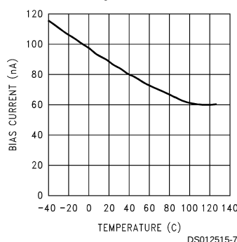
Feedback Pin Bias Current vs Temperature
