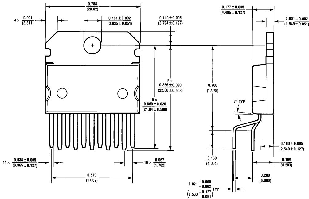
Molded TO-220 Package (TA) Order Number LM2984CT NS Package Number TA11A
