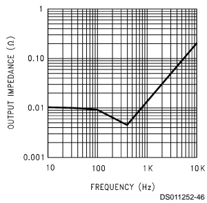
Output Impedance ( V_{OUT} )
