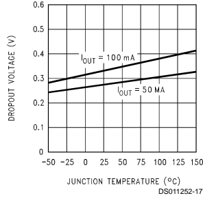
Dropout Voltage ( V_{buf} )
