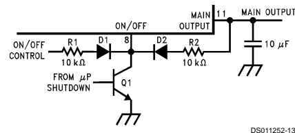
FIGURE 1. Power Down Override
