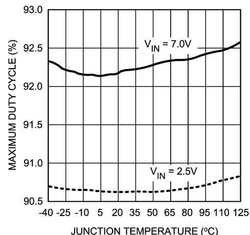
660kHz Max. Duty Cycle vs. Temperature
