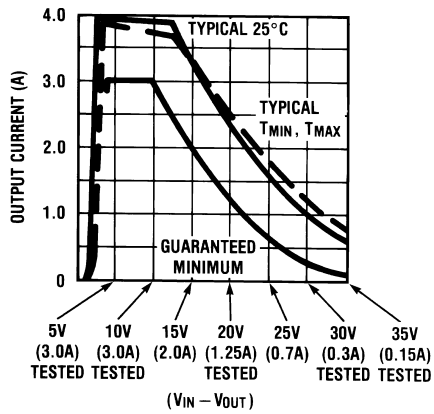
LM133 Guaranteed Output Current
