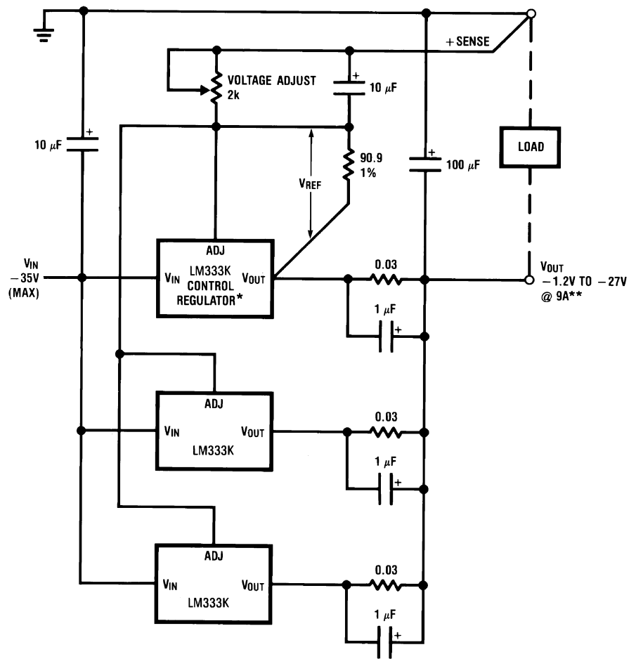
High-Current Adjustable Regulator
