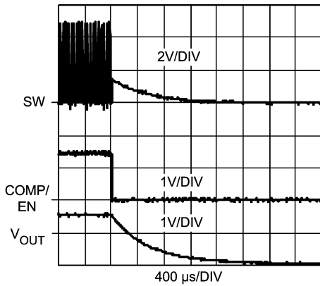
Shutdown R_{LOAD} = 1\Omega , V_{IN} = 5\text{V}
