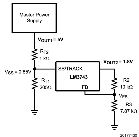
FIGURE 1. Tracking Circuit
