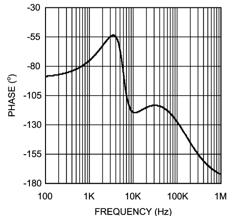
FIGURE 11. Overall Loop Gain and Phase
