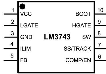
10-Lead Plastic MSOP NS Package Number MUB10A Top View
