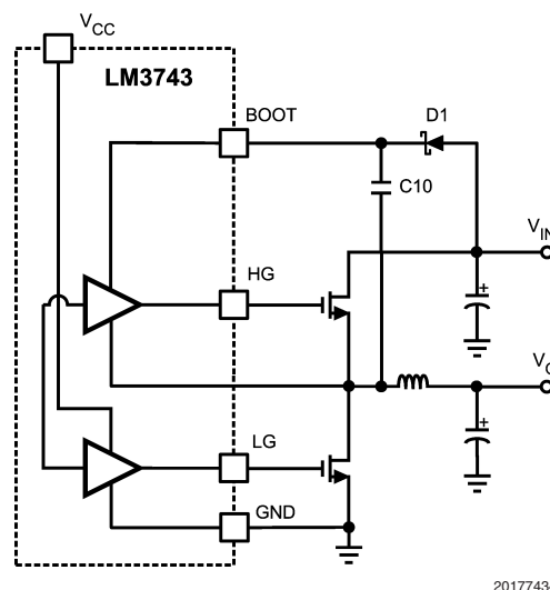
FIGURE 4. Charge Pump Circuit and Driver Circuitry
