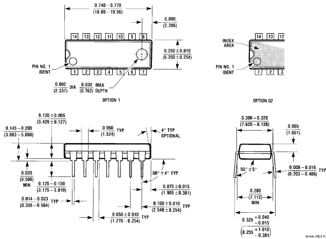
Molded Dual-In-Line Package (N) Order Number LM390N See NS Package Number N14A
