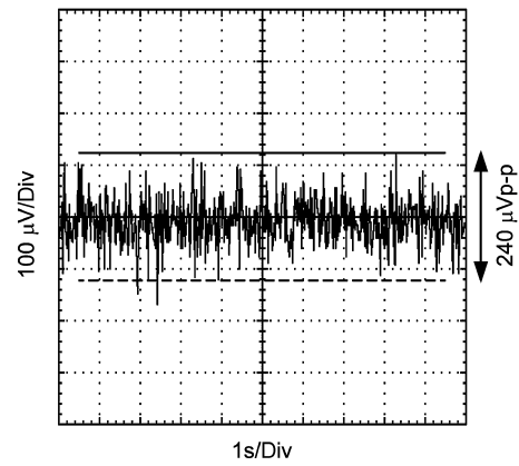
0.1 - 10 Hz Noise
