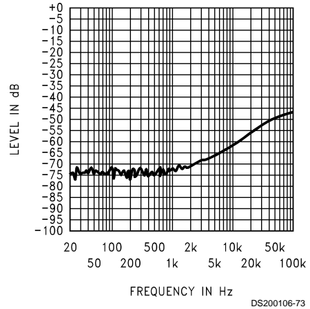
Input Floating
