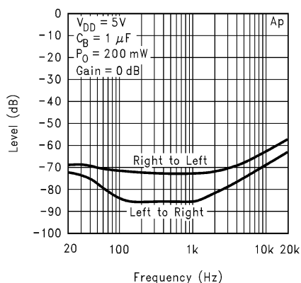
Power Amplifier Crosstalk
