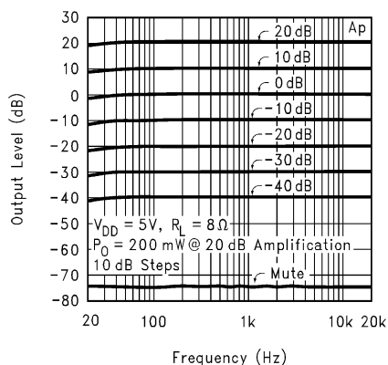
Power Amplifier Attenuation vs Frequency
