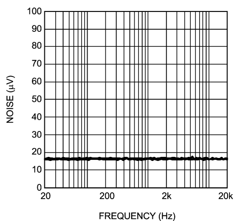
Noise V_{DD} = 3.3V , BTL, Mode 5, BTL
