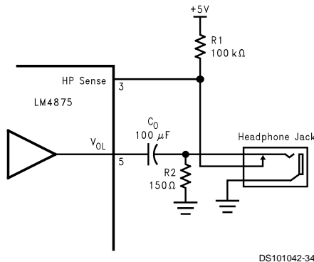
FIGURE 3. Headphone Circuit
