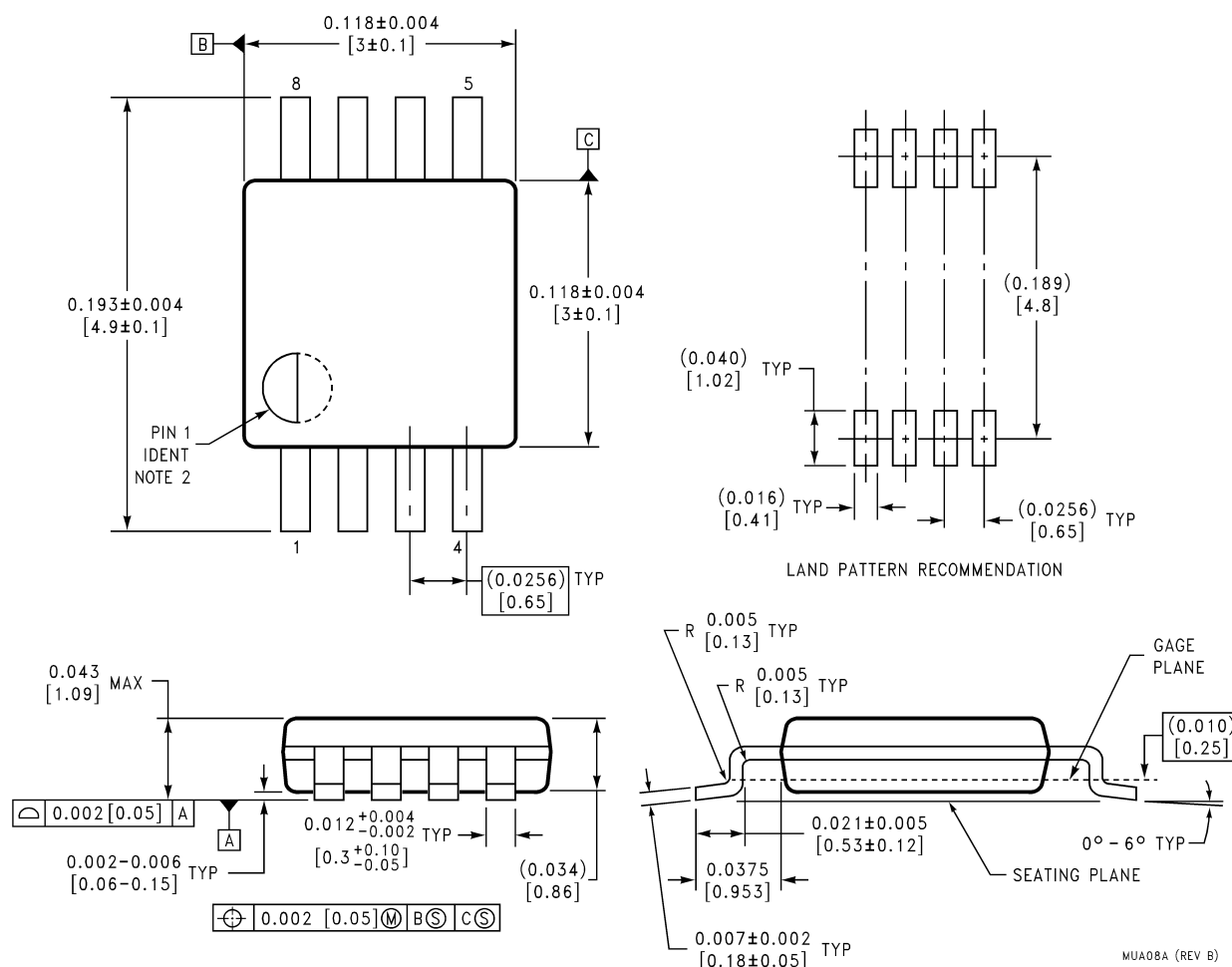
8-Lead (0.118' Wide) Molded Mini Small Outline Package Order Number LM4875MM NS Package Number MUA08A
