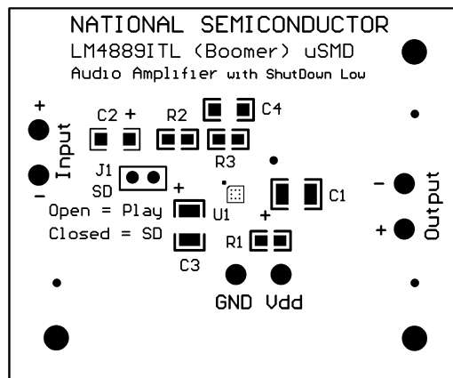
Silk Screen
