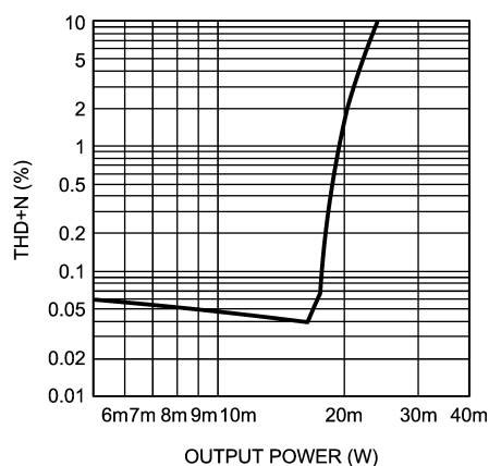
THD+N vs Output Power V_{DD} = 2.5V , R_L = 32\Omega C-CUPL
