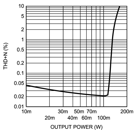
THD+N vs Output Power V_{DD} = 5.0V , R_L = 16\Omega C-CUPL
