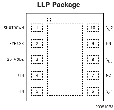
Top View Order Number LM4990LD See NS Package Number LDA10B
