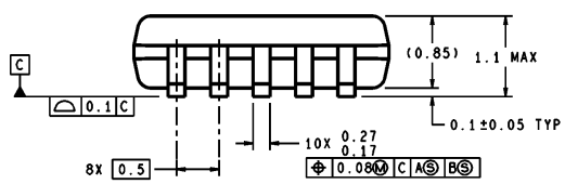
Exposed-DAP TSSOP Order Number LM4990MH NS Package Number MXF10A
