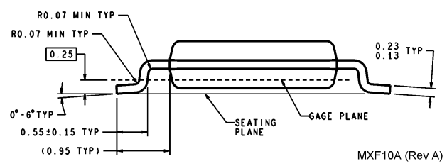
Exposed-DAP TSSOP Order Number LM4990MH NS Package Number MXF10A
