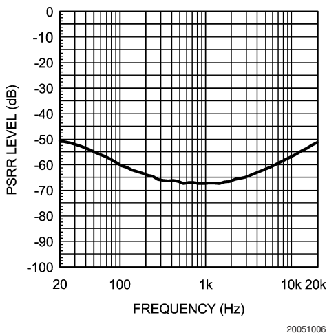
Power Supply Rejection Ratio (PSRR) vs Frequency V_{DD} = 5V, R_L = 8\Omega, \text{ input } 10\Omega \text{ terminated}
