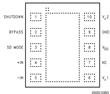
Top View Order Number LM4990LD See NS Package Number LDA10B
