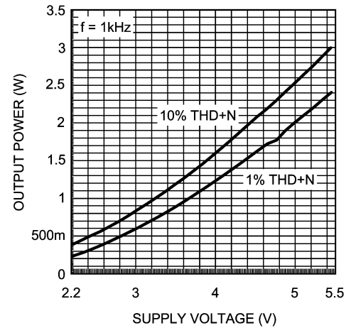
Output Power vs Supply Voltage, R_L = 4\Omega
