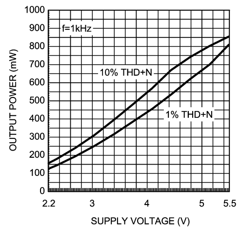
Output Power vs Supply Voltage, R_L = 16\Omega
