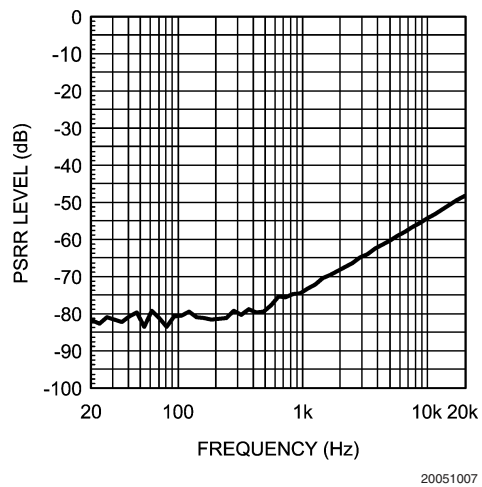
Power Supply Rejection Ratio (PSRR) vs Frequency V_{DD} = 5V, R_L = 8\Omega, \text{ input floating}
