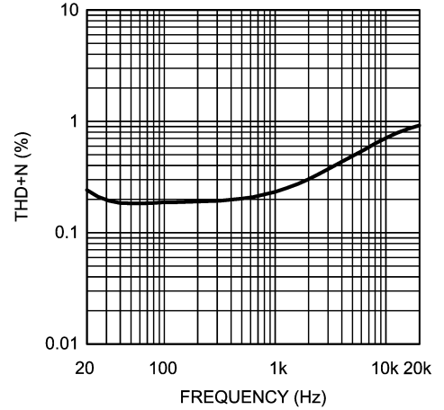
THD+N vs Frequency V_{DD} = 2.6V , R_L = 4\Omega , and P_O = 150mW
