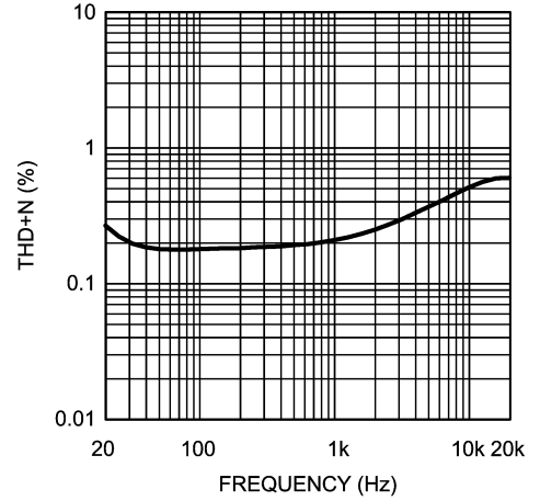
THD+N vs Frequency V_{DD} = 3V , R_L = 4\Omega , and P_O = 500mW
