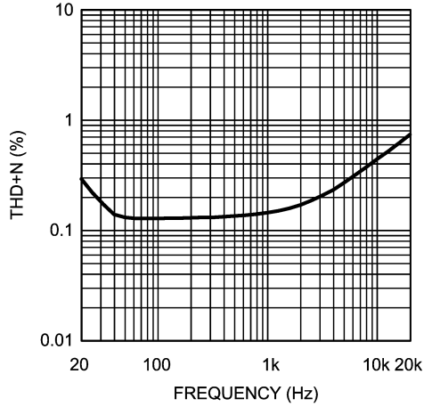
THD+N vs Frequency V_{DD} = 5V , R_L = 8\Omega , and P_O = 500mW
