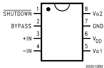
Top View Order Number LM4990MM See NS Package Number MUA08A
