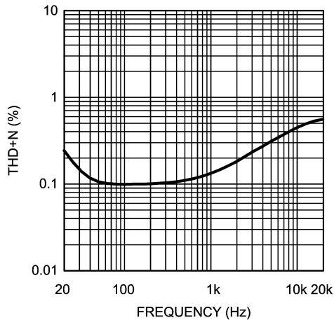
THD+N vs Output Power V_{DD} = 2.6V , R_L = 8\Omega , and P_O = 150mW
