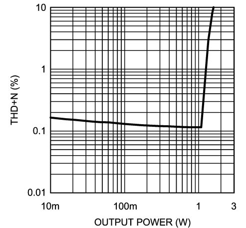
THD+N vs Output Power V_{DD} = 5V , R_L = 8\Omega , and f = 1kHz
