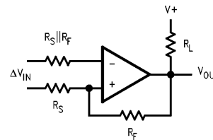
FIGURE 4. R_S and R_F Add Hysteresis to Comparator
