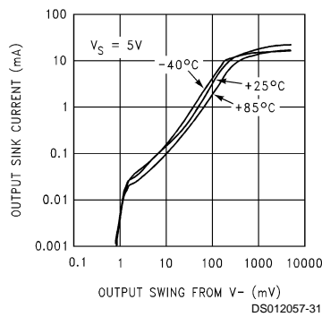
Output Voltage vs Sink Current
