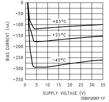
Bias Current vs Supply Voltage
