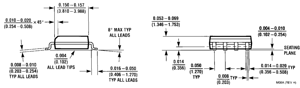
8-Pin Small Outline Package Order Number LM6142AIM, LM6142AIMX or LM6142BIM, LM6142BIMX NS Package Number M08A
