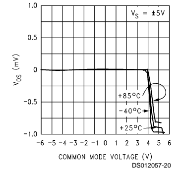
Offset Voltage vs V_{CM}
