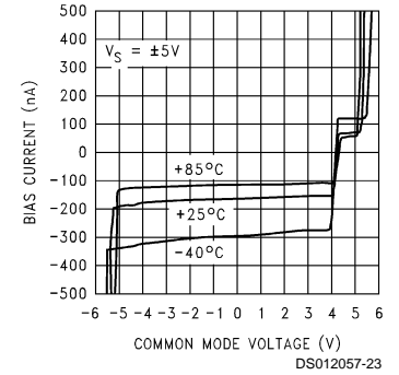
Bias Current vs V_{CM}
