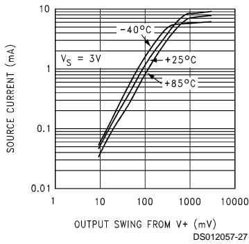
Output Voltage vs Source Current
