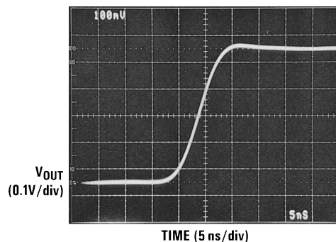
FIGURE 1. 1a, 1b: Variation of Closed Loop Gain from -1 to -5 Yields Similar Responses
