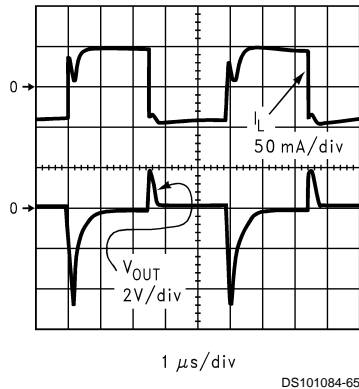
FIGURE 9. V_{com} driver performance scope photo
