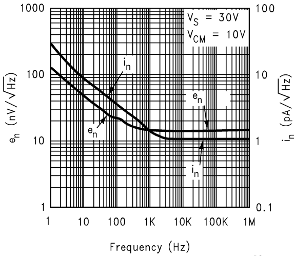
Input Noise Voltage/Current vs. Frequency
