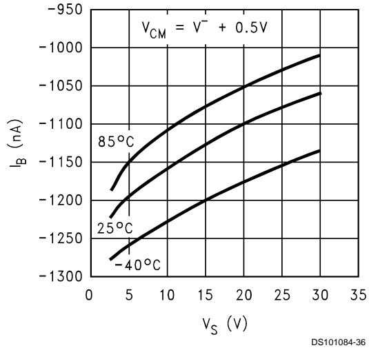
I_B vs. V_S
